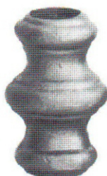
DHP14-09 H 70 mm W Ø 42 mm Ø 20.5 mm 0.355 kg $4.20ea
