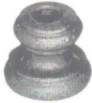
DHP14-03 H 40 mm W Ø 40 mm Ø 20.5 mm 0.180 kg $2.40ea
