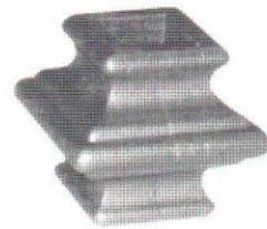
DHP14-06 H 45mm W Ø 47mm Ø 16.5 mm 0.350 kg $2.60ea
